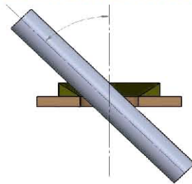
Maximum Off-Axis Entry Angle for DPM Fiberglass Fittings and Common Pipes
