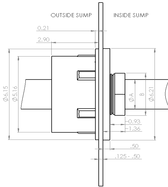
Compact Fitting for Corrugated Duct Application
